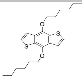
4,8-dihexyloxybenzo[1,2-b:4,5-b']dithiophene
