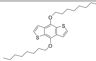
4,8-dioctyloxybenzo[1,2-b:4,5-b']dithiophene
