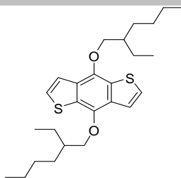
4,8-Bis(2-ethylhexyloxy) benzo[1,2-b:4,5-b']dithiophene
